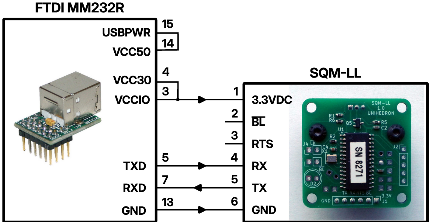
Figure 5.2: SQM-LLtest setup
